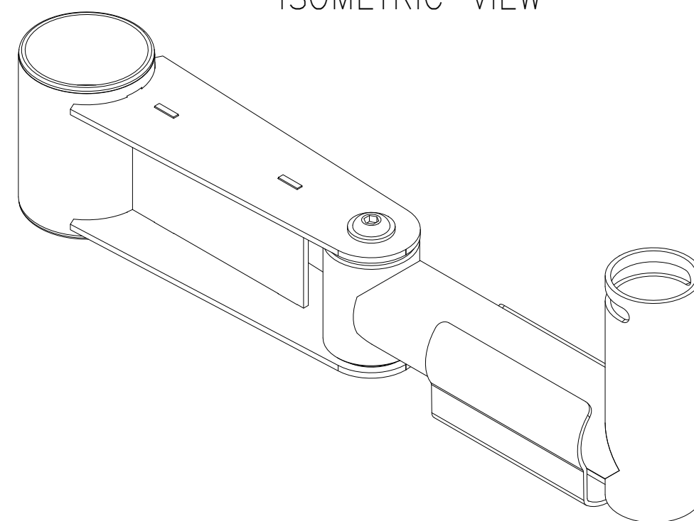
ISOMETRIC VIEW
