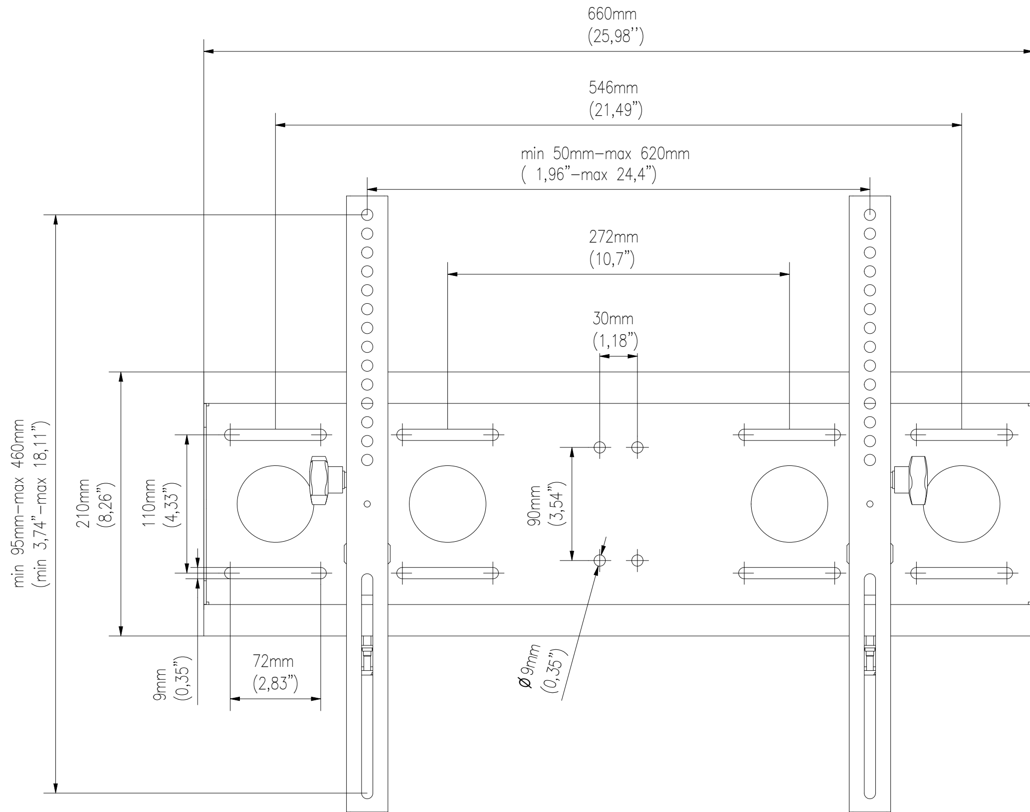
FRONT VIEW
