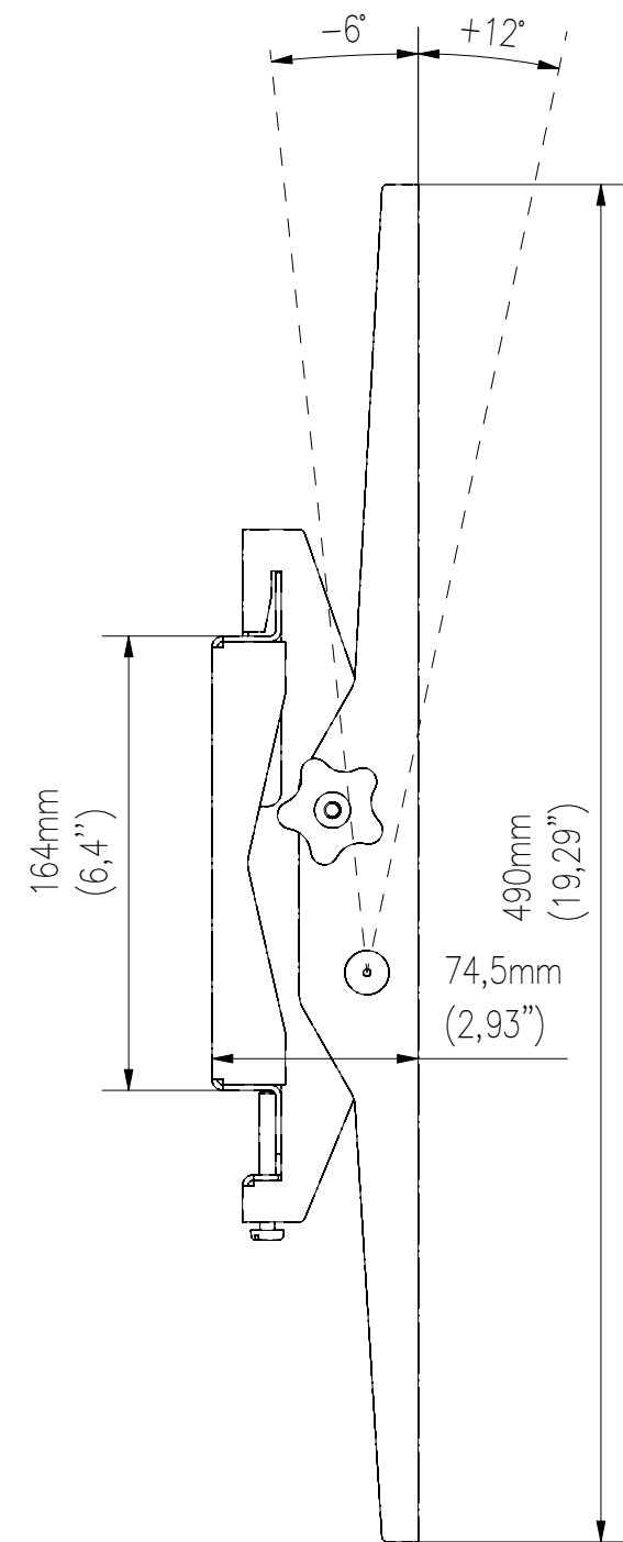
SIDE VIEW
