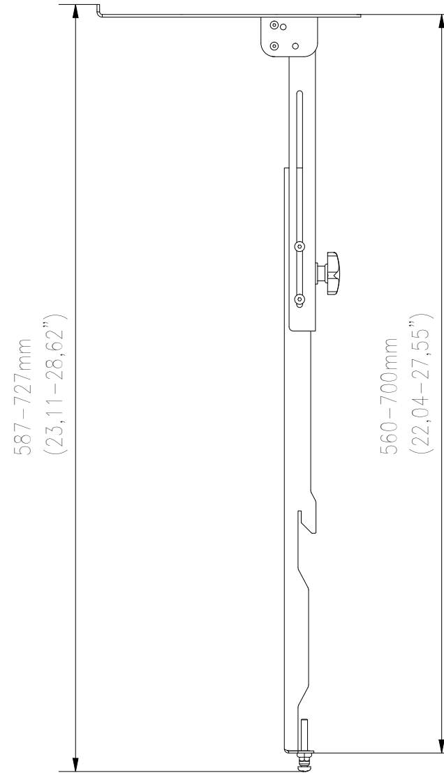
SIDE VIEW
