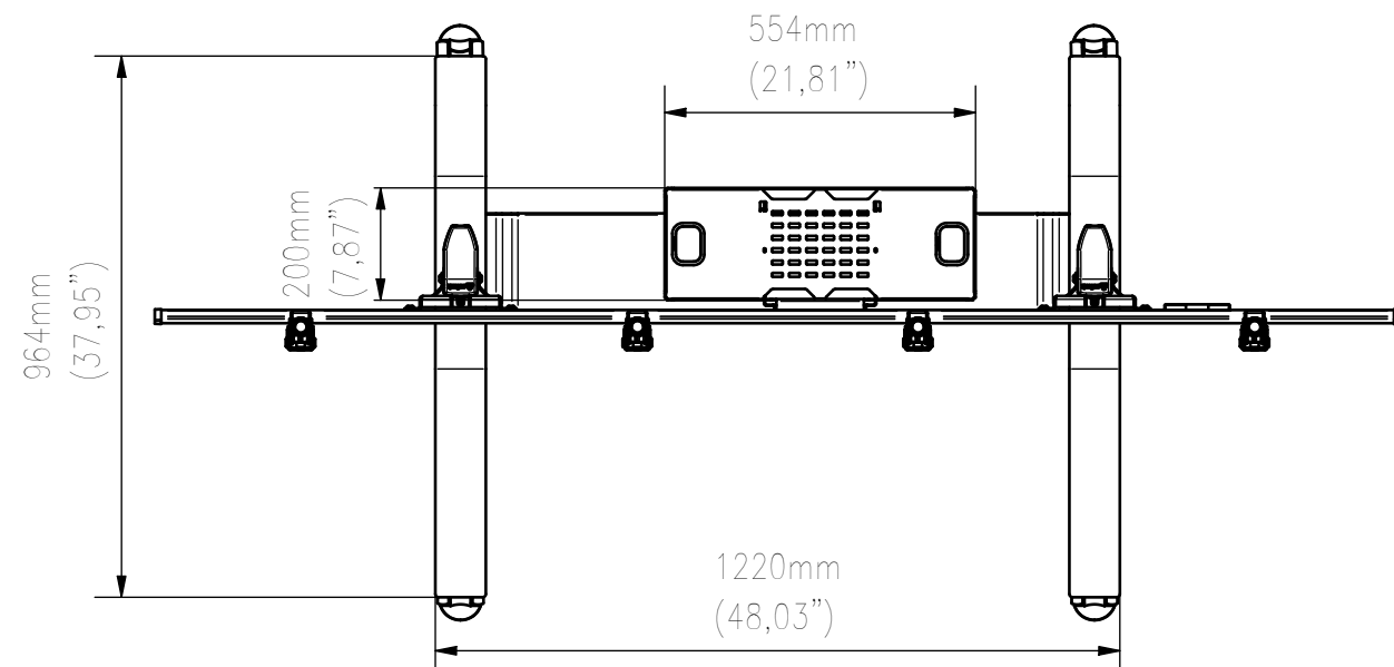
TOP VIEW
