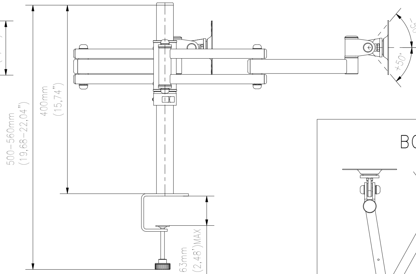
SIDE VIEW
