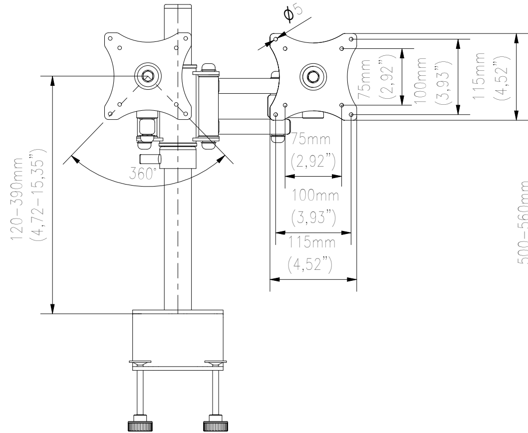
FRONT VIEW
