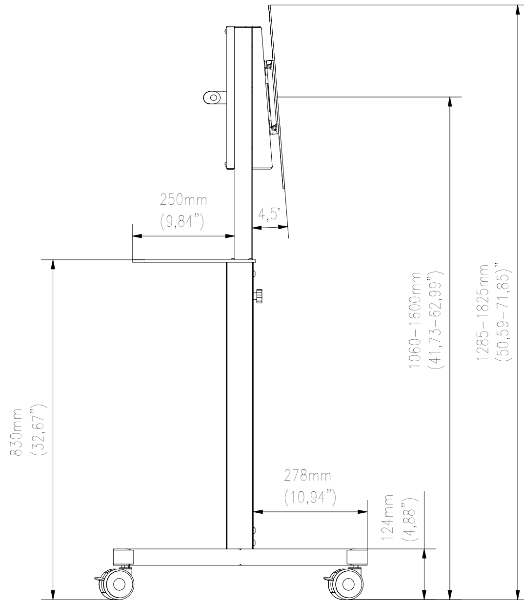
SIDE VIEW
